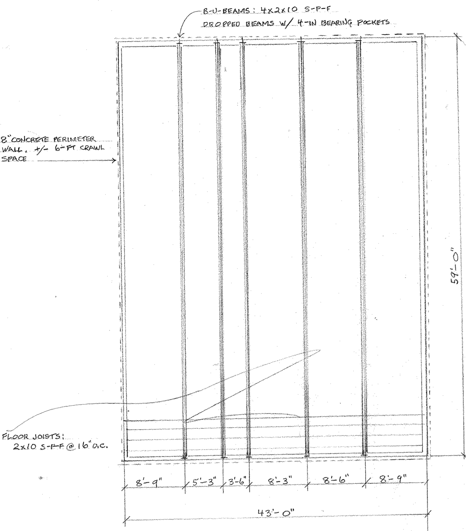
3 A-1 FLOOR FRAMING SCALE 1/8" = 1'-0"
